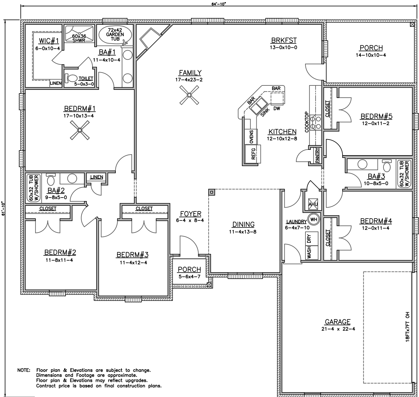
FLOOR PLAN
