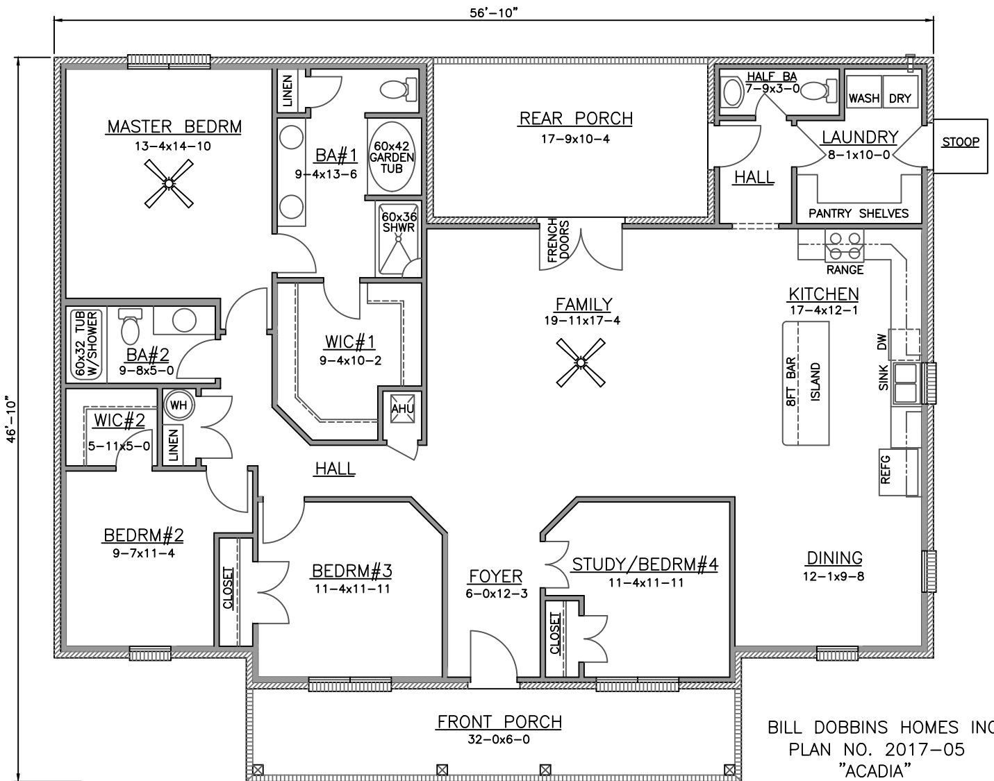
FLOOR PLAN
