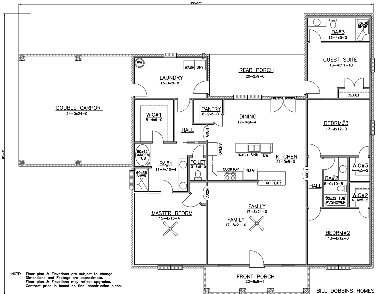
FLOOR PLAN
