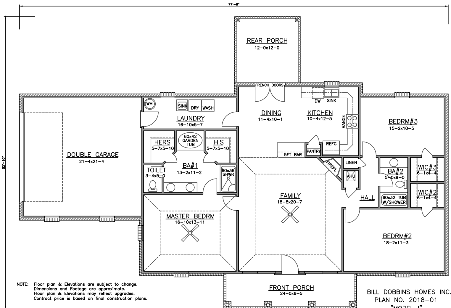
FLOOR PLAN
