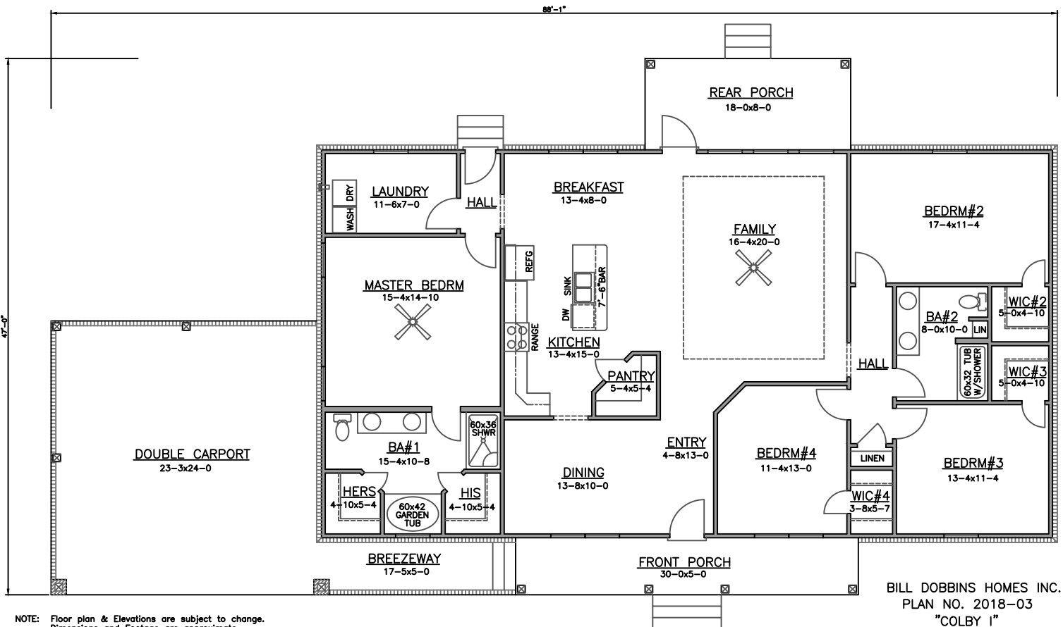
FLOOR PLAN
