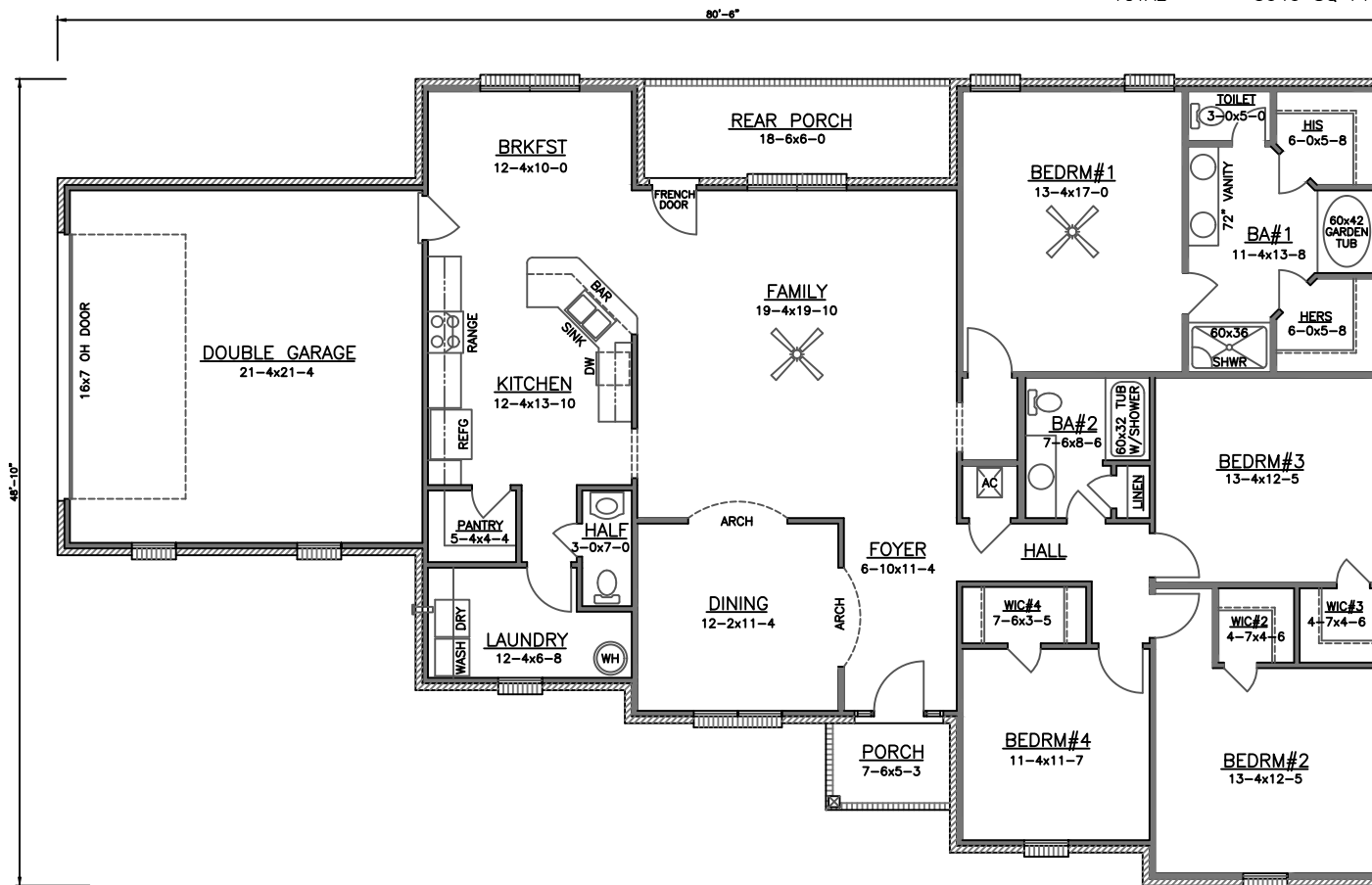
FLOOR PLAN
