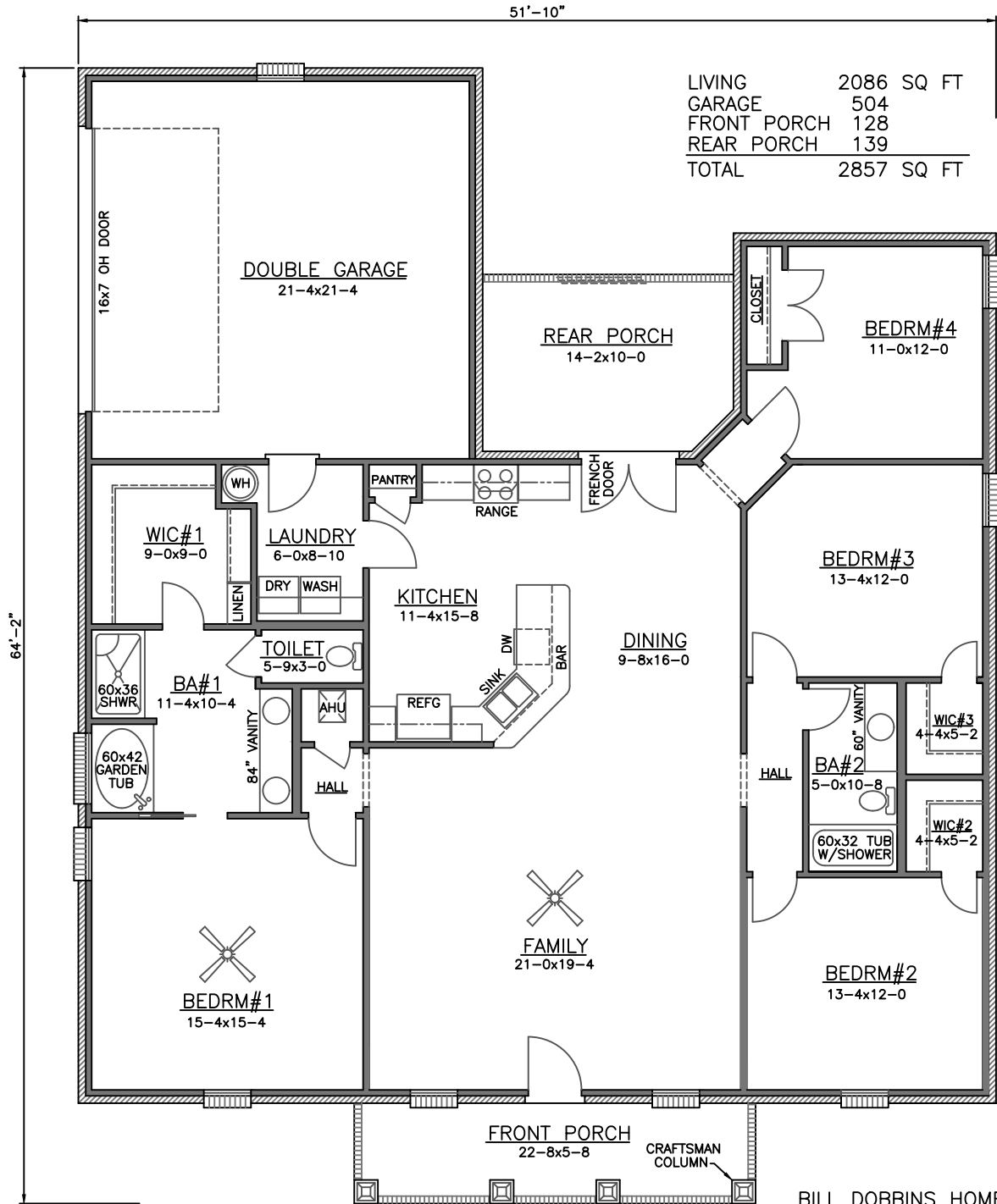
FLOOR PLAN
