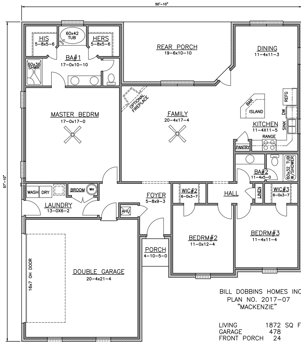
FLOOR PLAN
