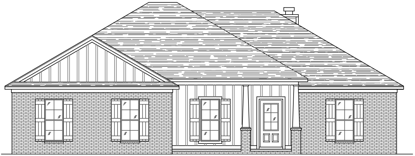
FRONT ELEVATION
