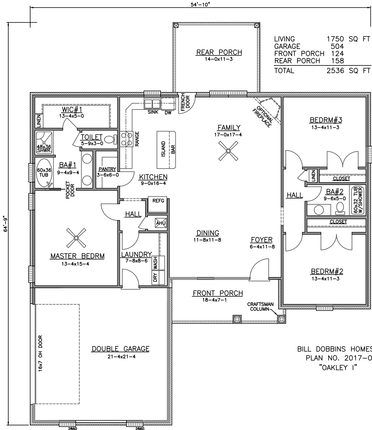
FLOOR PLAN
