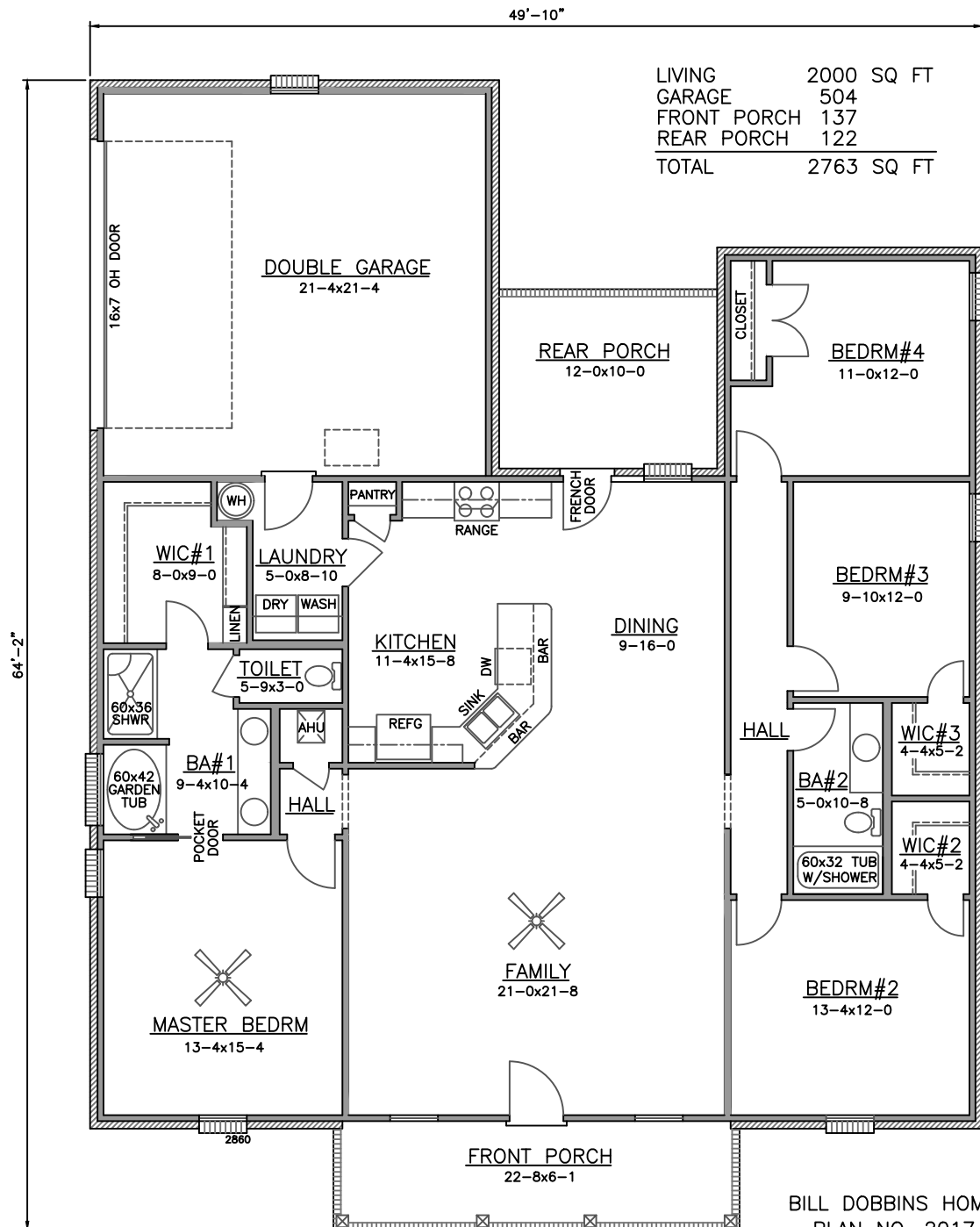
FLOOR PLAN
