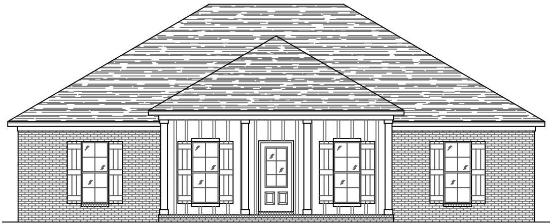
FRONT ELEVATION
