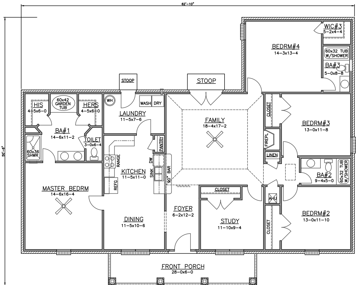
FLOOR PLAN
